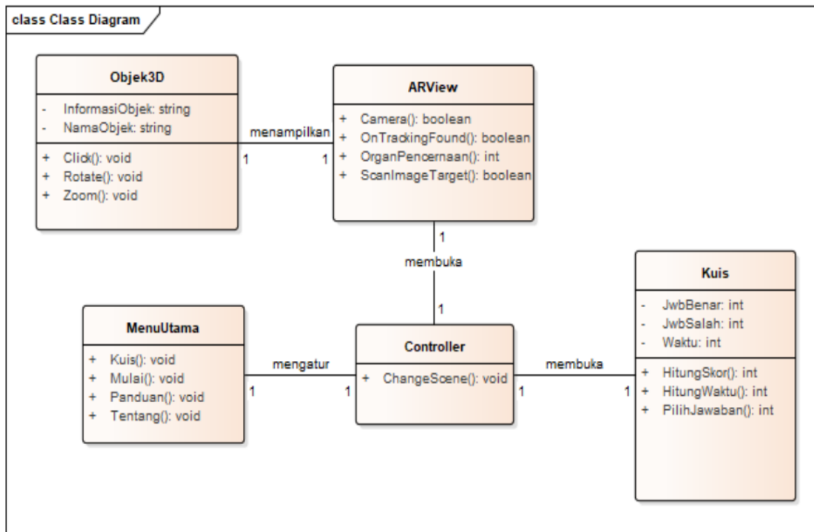
Figure 4. "ARSIPERSIA" class diagram
