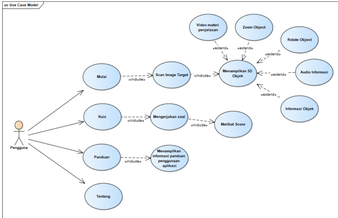
Figure 3. "ARSIPERSIA" use case diagram
