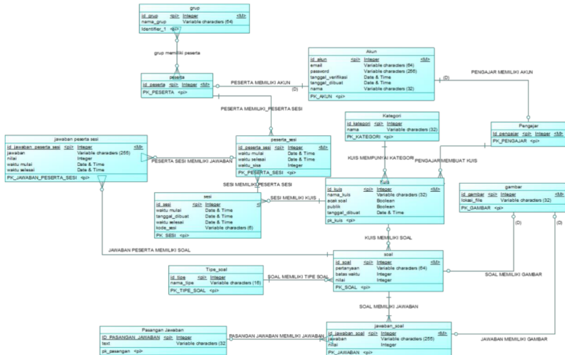
Gambar 5. Conceptual Data Model Website Kuisin
