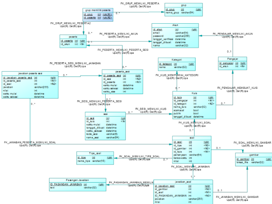
Gambar 6. Physical Data Model Website Kuisin
