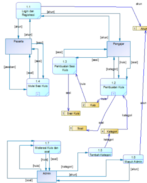
Gambar 3. DFD Level 1 Website Kuisin
