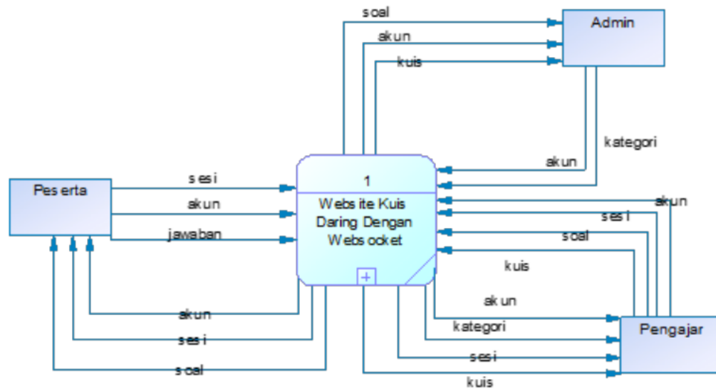
Gambar 2. Context Diagram Website Kuis Daring
