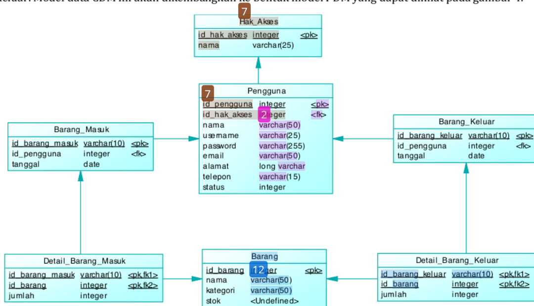
Gambar 4. Physical Data Model
