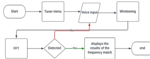
Figure 3. Tuner flowchart
