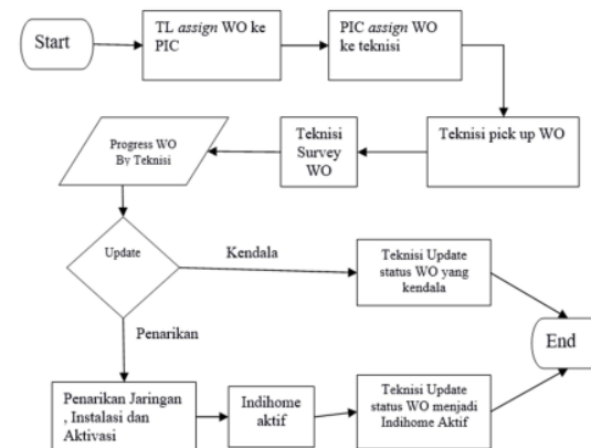
Gambar 1. Proses Monitoring Work Order
